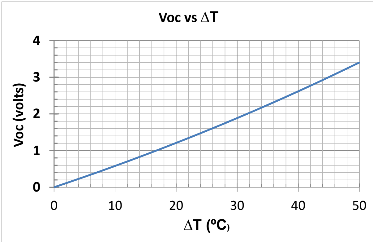
Figure 1 – Open Circuit (No Load) Voltage vs \Delta T for the TXL-127-02K
