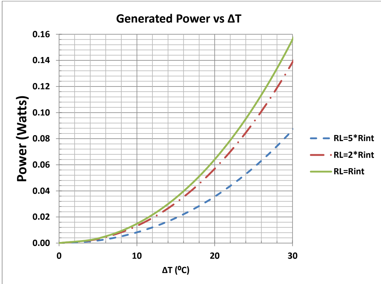
Figure 4 – Load Power as a Function of \Delta T for Three Different Load Resistances Using a TXL-127-02K Module
