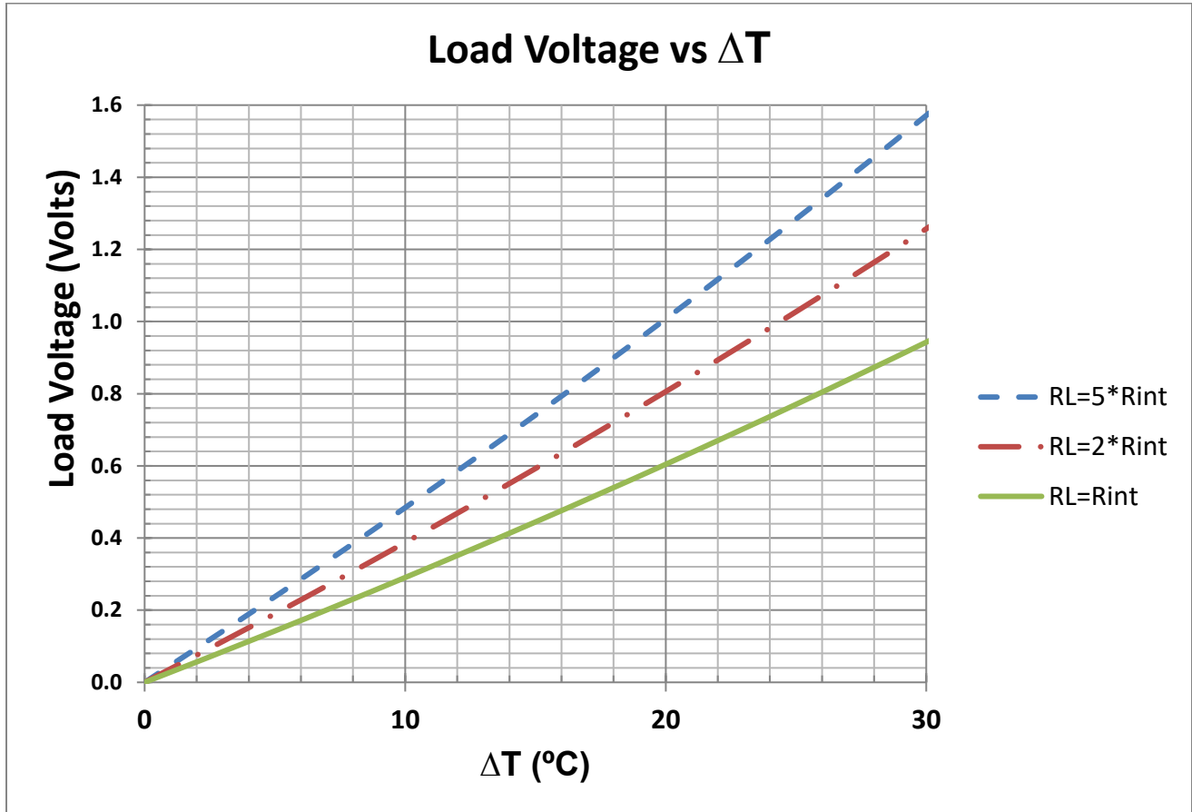
Figure 3 – Load Voltage as a Function of \Delta T for Three Different Values of Load Resistance for the TXL-127-02K
