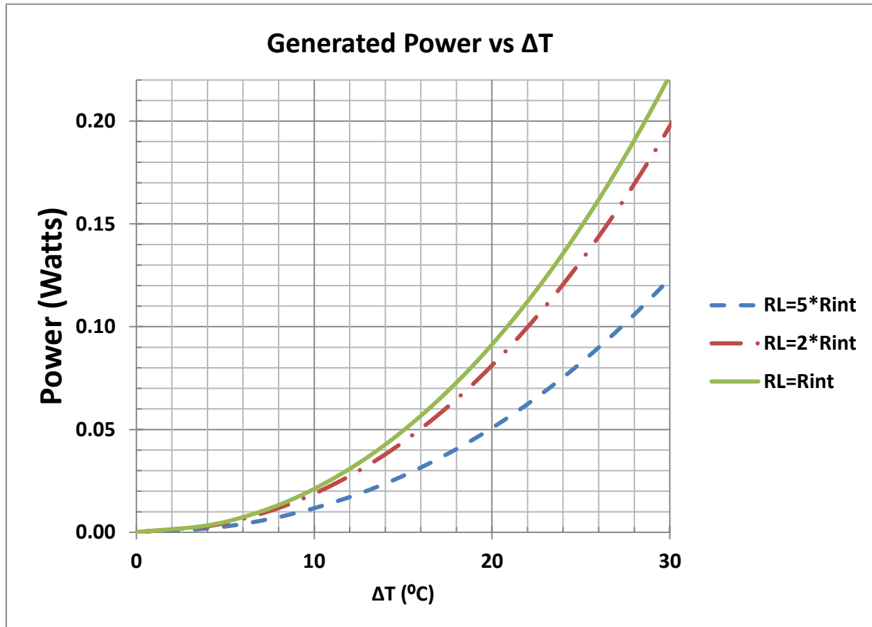
Figure 4 – Load Power as a Function of \Delta T for Three Different Load Resistances Using a TXL-127-03L Module
